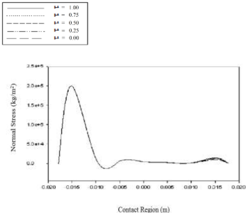
Figure 5. Normal stress inside the contact region.
