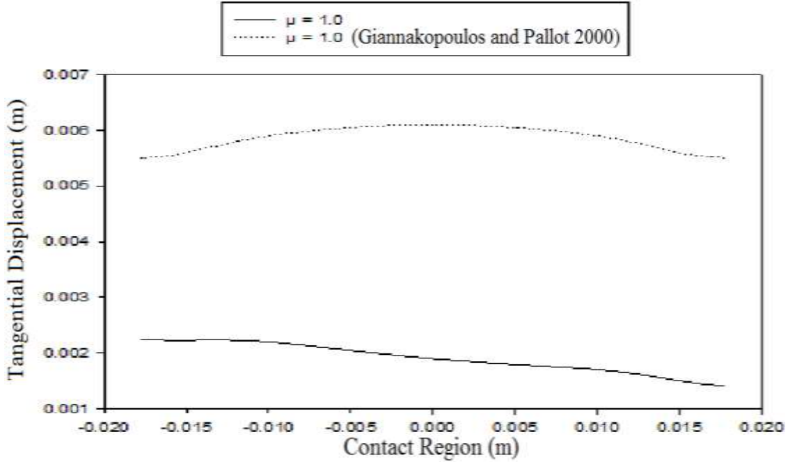
Figure 11. The comparison of the tangential displacement between the Giannakopoulos and Pallot’s method and the method that is used in this study.
