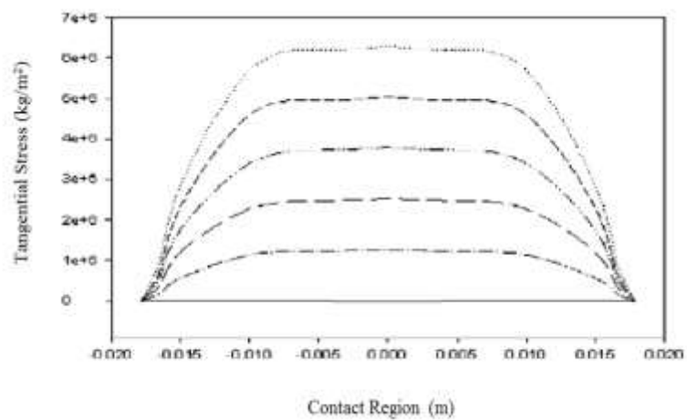
Figure 4. Tangential stress inside the contact region.
