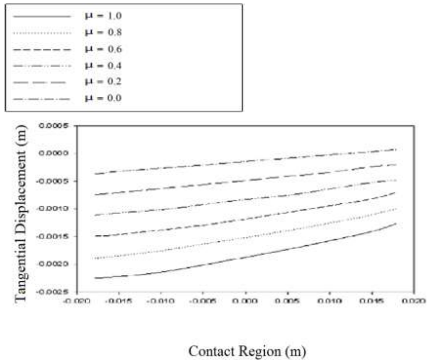
Figure 8. The tangential displacement in contact region.
