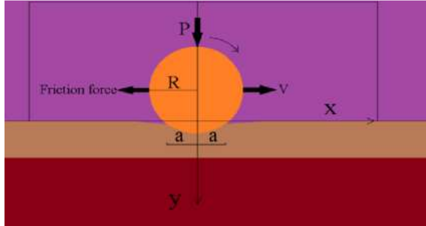
Figure 1. Coordinates system that is assumed in contact of roller with half space.
