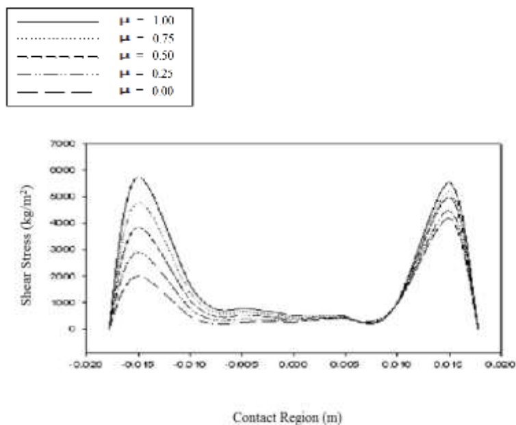
Figure 6. Shear stress inside the contact region.
