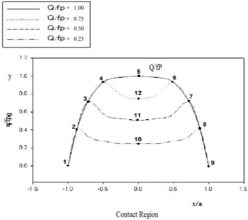
Figure 7. Tangential stress inside the partial slip contact region.
